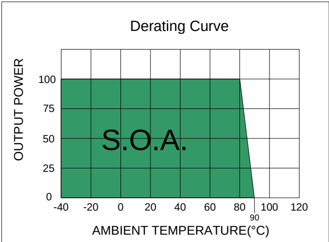
24V input and Efficiency < 85%
